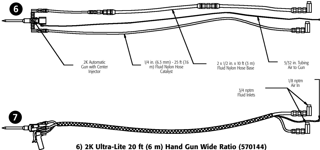
6) 2K Ultra-Lite 20 ft (6 m) Hand Gun Wide Ratio (570144) 7) 2K Ultra-Lite 20 ft (6 m) Hand Gun Close Ratio (570091)
