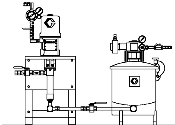
J) 10 gal. (38 liter) Press Tank with 15:1 Booster (570037)
