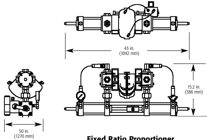
Fixed Ratio Proportioner
