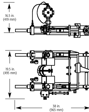
Variable Ratio Proportioner
